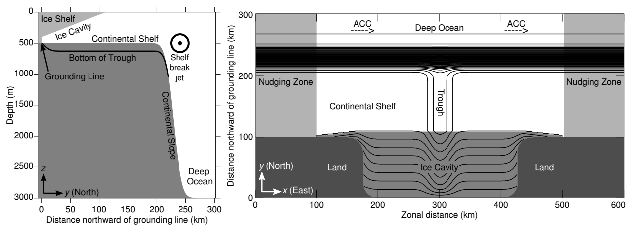
FIG. 1. Geometry of the idealized ice shelf-coastal domain. (Left) Side view. (Right) Top view. The contour lines are the thickness of the water column (interval 50 m).
