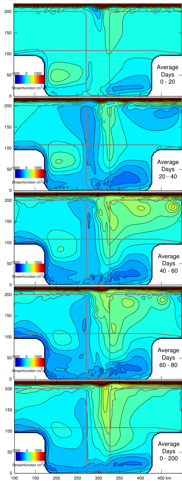
FIG. 11. As in Fig. 5 but for the case with a shelf break jet and thermodynamics (Run #7).
