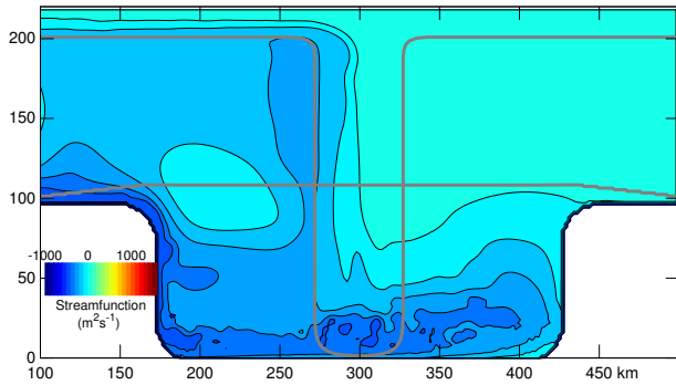
FIG. 5. Mean circulation over the deep isopycnal \gamma_2 in the case with a trough and no shelf break jet (Run #2). The contour interval for the streamfunction \psi is 10^2 \text{ m}^2 \text{ s}^{-1} and the flow is to the right of \nabla \psi . The gray lines give the extent of the trough and that of the ice shelf.
