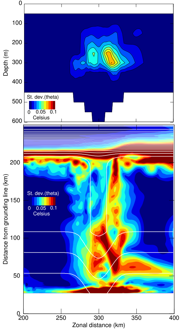
FIG. 14. (Top) Standard deviation of potential temperature \theta across the plane y = 155 km. The 'steps' in the bathymetry are plotting artefacts and the model bathymetry is actually smooth. (Bottom) Same as above but at 300 m. White contour lines are water column thickness (interval 100 m). Results are averaged over days 153–279 (Run #7).
