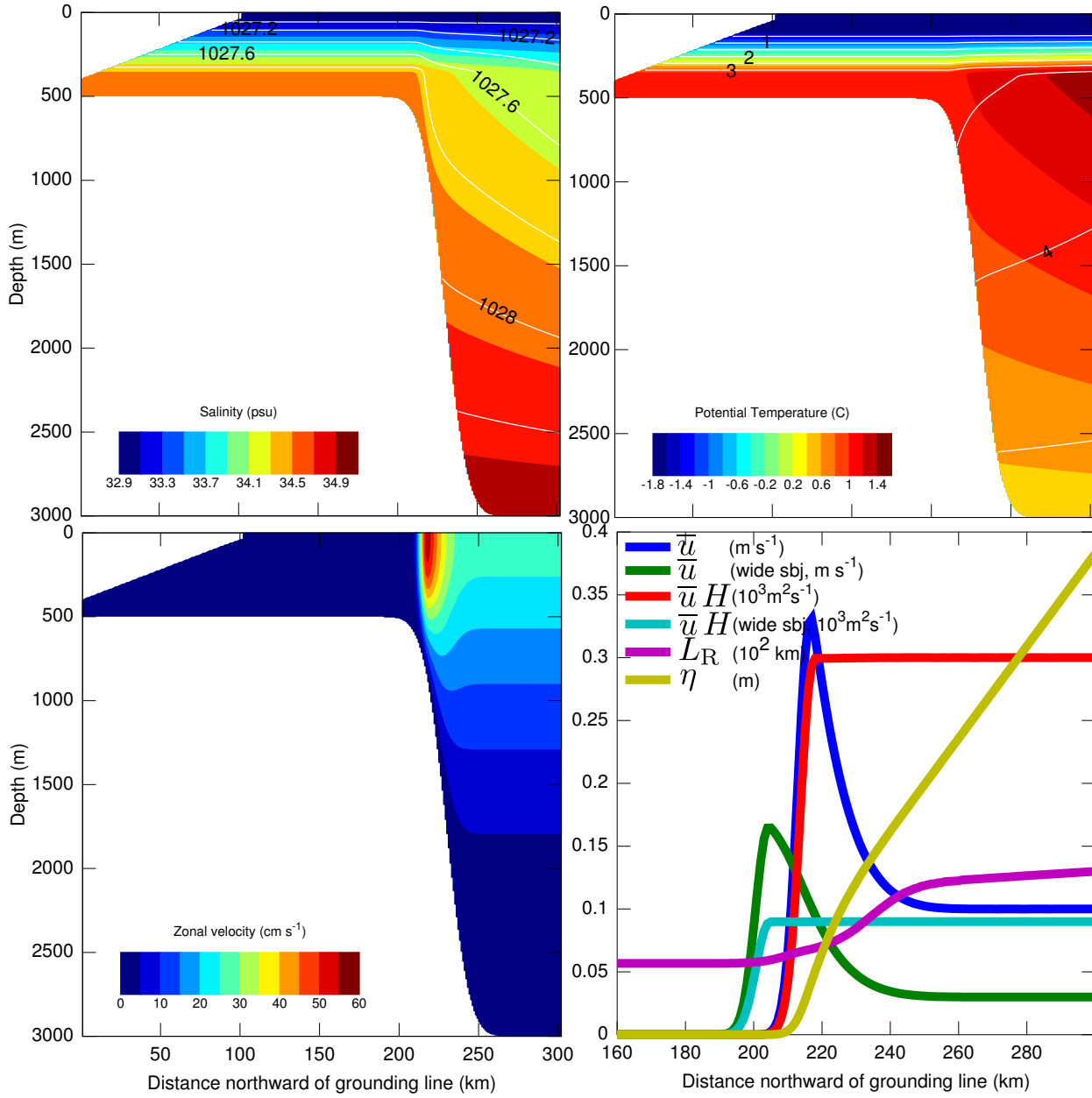
FIG. 2. Initial and boundary conditions used in Runs #1,5,6,7,11. (Top left) Salinity S and neutral density \gamma (contour lines). (Top right) Potential temperature \theta and temperature T above in situ freezing point (contour lines). (Bottom left) Zonal velocity (positive eastward/out of the page). (Bottom right) Cross-shelf variation of various parameters. See text for definition of symbols.
