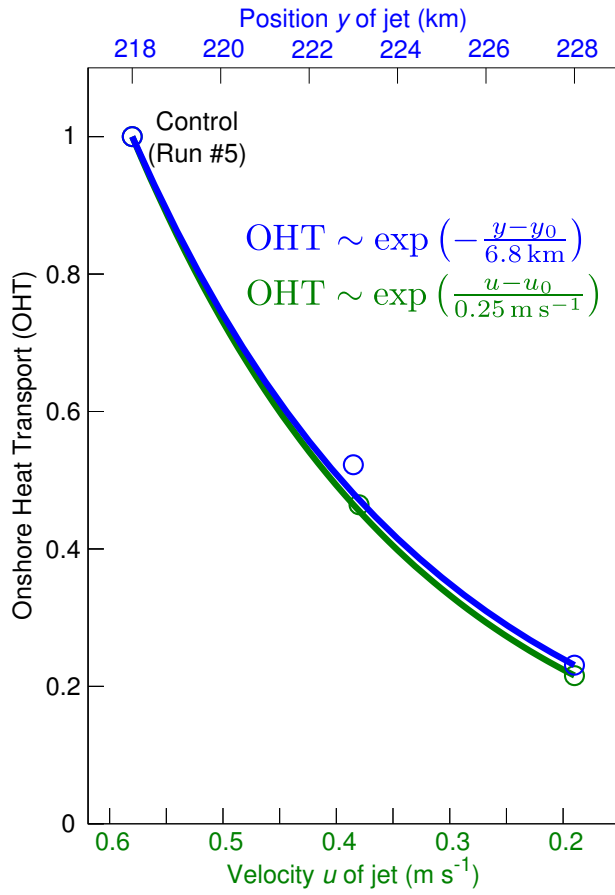
FIG. 10. Sensitivity of mean Onshore Heat Transport (OHT) to the position and velocity of the jet (Mechanism 3; Runs #5,13–16). The transport is non-dimensionalized by its value from the control simulation (Run #5). The solid lines are exponential regressions to the data points. The Rossby radius of deformation is 6.9 km at y = 220 km.
