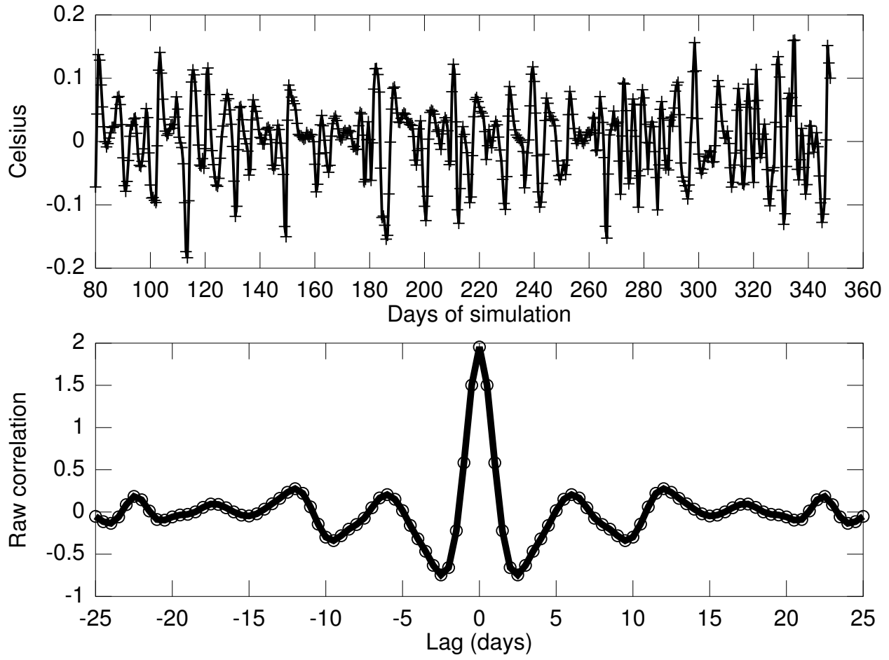
FIG. 12. (Top) Temperature anomaly at 300 m at the entrance of the trough. The sampling interval is 0.5 days. (Bottom) Lagged-correlation of the temperature anomaly timeseries with itself. Correlation is high for lags T_i = \pm 6.5n days with n = 0, 1, 2, \dots
